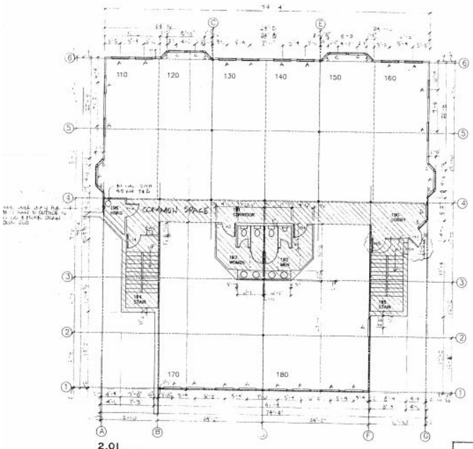
2.01 FIRST FLOOR PLAN SCALE: 1/8" = 1'-0"
