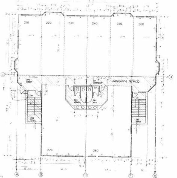
2.02 SECOND FLOOR PLAN SCALE: 1/8" = 1'-0"
