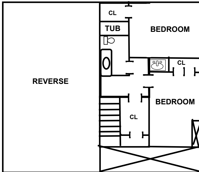
22 Anthony Drive FLOOR PLAN
