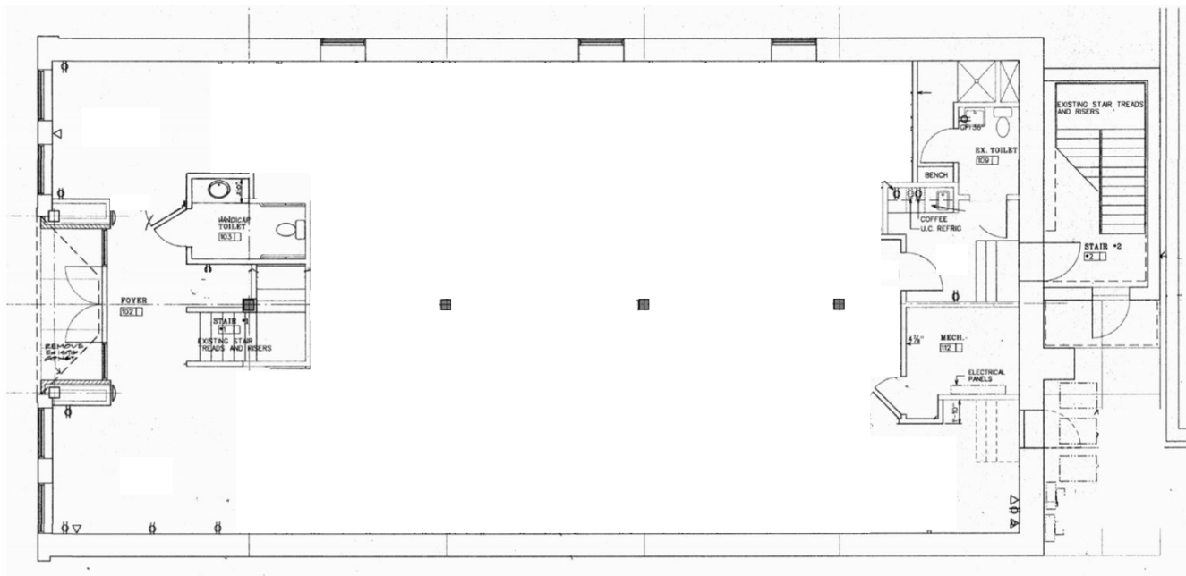
First Floor
